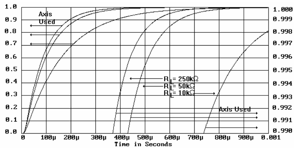
Figure 4 - 100μA Range, R_M = 50k\Omega
