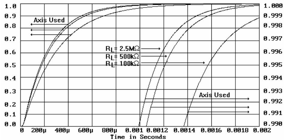
Figure 5 - 10μA Range, R_M = 500k\Omega
