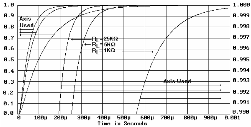
Figure 3 - 1mA Range, R_M = 5k\Omega
